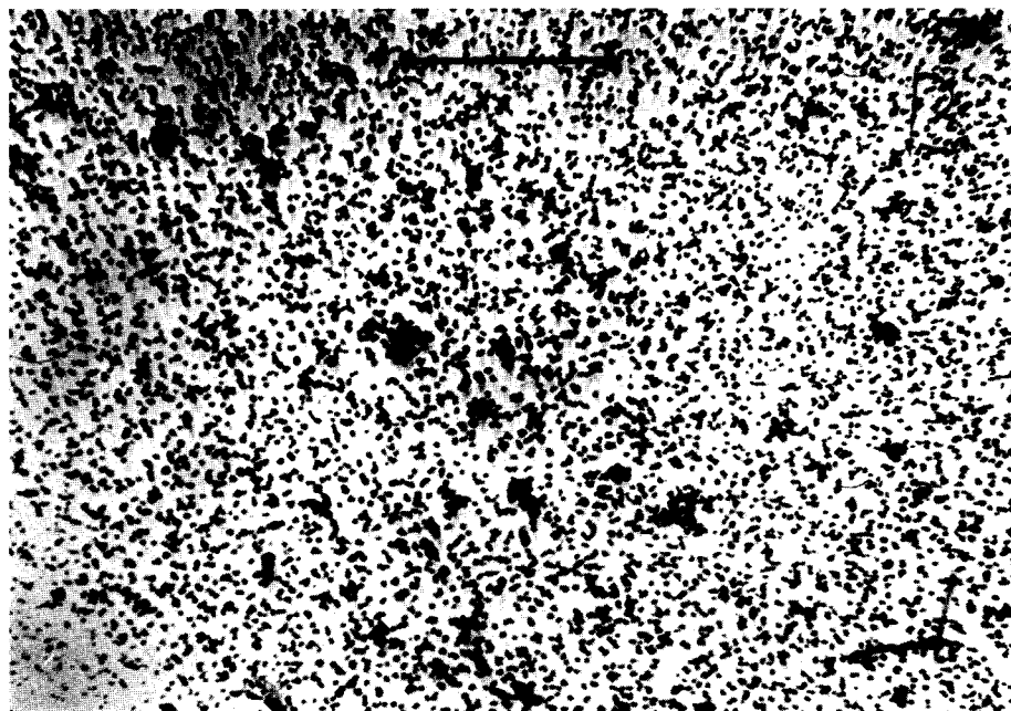
Fig. 5. Microphotographs of the surfaces of spalls of potassium sulphate containing 50 m-curie of sulphur-35 (pure \beta -emitor).
