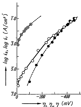
Fig. 8. \log i_s-\eta_s , \log i_s-\eta_{1s} and \log i_1-\eta relations in 0.1N NaOH.
