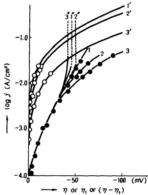
Fig. 3. \log j plotted against \eta (1, 2, 3), or \eta_1 (1', 2', 3') or \eta-\eta_1 (1'', 2'', 3'') on Au plate at 23°C in sulfuric acid: 1.3N(1, 1', 1''), 0.67N(2, 2', 2''), 0.3N(3, 3', 3'').
