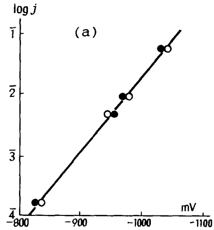
Fig. 2. \log j plotted against \eta (●) or \eta_1 (○) on liquid Ga in aqueous 0.1N NaOH at 31°C.
