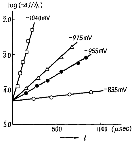
Fig. 1. \log(-\Delta j/\eta_1) vs. time curves on liquid Ga in 0.1N NaOH at 31°C, obtained from the transient curves which started from different values of steady state overvoltage.
