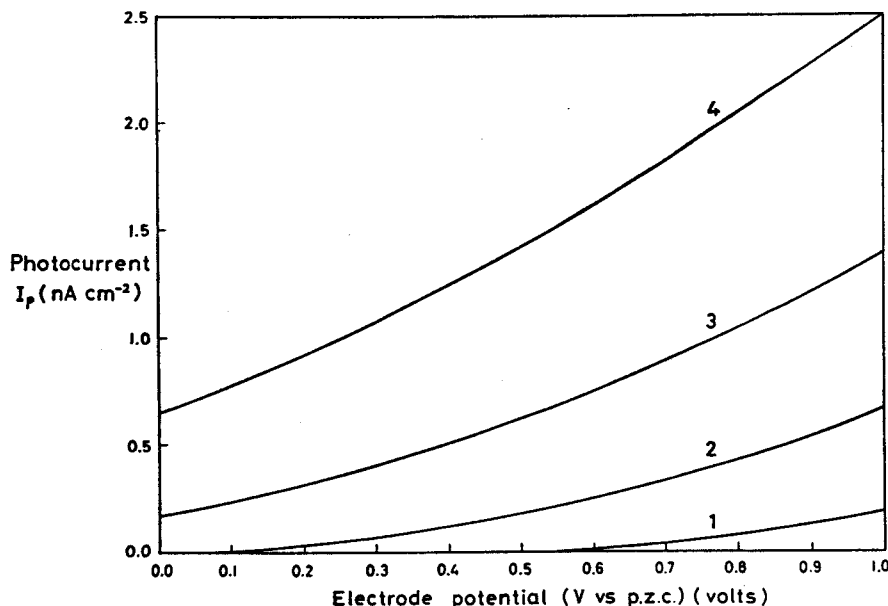
Fig. 6. The dependence of the photocurrent on electrode potential for electron transfer from a mercury electrode to acceptors in the electrolyte for different incident photon energies, h\nu . Curve 1, for h\nu=2.5 eV. Curve 2, for h\nu=3.0 eV. Curve 3, for h\nu=3.5 eV. Curve 4, for h\nu=4.0 eV.
