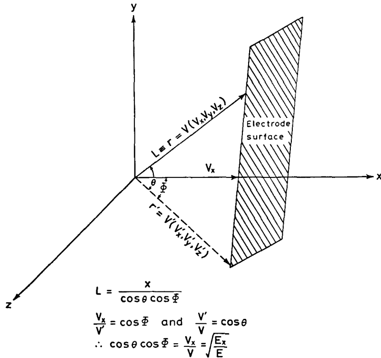
Fig. 4. Vectorial representation of the angular distribution of the electrons which move towards the metal surface from within the bulk when stimulated by light.
