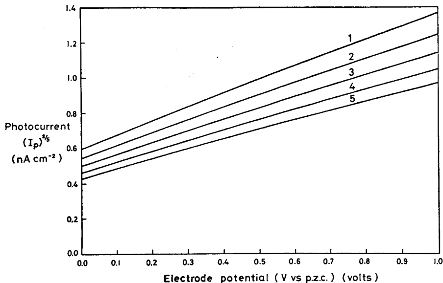
Fig. 8. The dependence of 2/5th power of the photocurrent on electrode potential for electron transfer from a mercury electrode to acceptors in the electrolyte for photon energy, h\nu=3.5 eV and for different barrier heights U_m . Curve 1, for U_m=13.8 (1.0 eV less than the calculated U_m=14.8 eV). Curve 2, for U_m=14.3 eV. Curve 3, for U_m=14.8 eV (calculated value). Curve 4, for U_m=15.3 eV and curve 5, for U_m=15.8 eV (1.0 eV more than the calculated U_m=14.8 eV).
