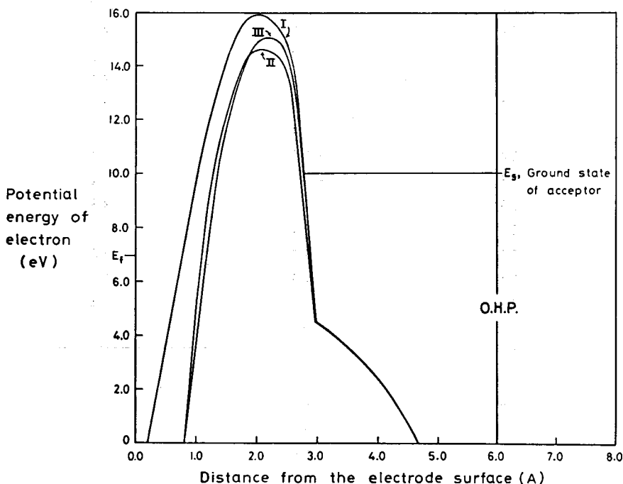
Fig. 5. Schematic diagrams of potential energy barrier for three typical paths of electron as shown in Fig. 1. I, for the electron path when y=0.0\text{Å} . II, for the electron path when y=0.7\text{Å} . III, for the electron path when y=1.5\text{Å} .
