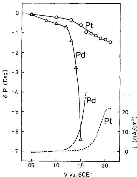
Fig. 5. Change in P and current density with potential for Pt (O, ---) and Pd ( \Delta , --) in 0.5 M aqueous acetate solution.
