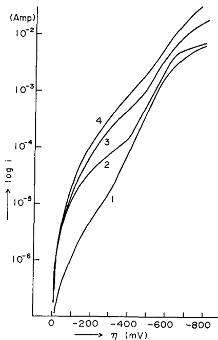
Fig. 1. Polarization curves of hydrogen evolution reaction on Ti in sulfuric acid at 23°C.
