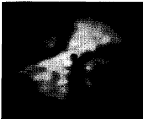
Fig. 1. Spotty and bright MoO 3 -clusters, caused to develop on a clean Mo-tip surface under the conditions, T=1000 K, P_{O_2} \sim 10^{-5} Torr and negatively applied high field of about 3 \times 10^7 V/cm. In this plate, the probe hole of 1-mm \phi in the screen is visible at the constricted part of the bright region, prominently around the {111} planes, which is a throng of granular MoO 3 -clusters.
