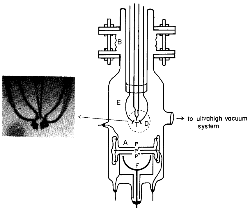
Fig. 3. A schematic diagram of the experimental setup. B: bellows arrangement, E: emitter tip assembly, T: Mo-tip, D: MoO 3 -cluster, A: van Oostrom type analyser, P: 1-mm \phi probe hole in the anode (screen), P' and P'': 2-mm \phi and 4-mm \phi probe holes in the lens-electrodes, F: Faraday cup.
