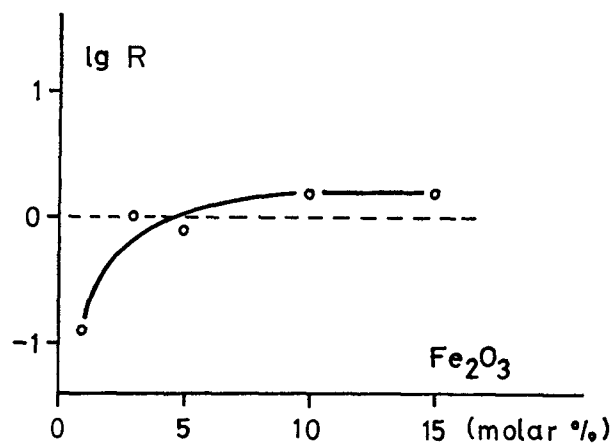
Fig. 6. Logarithm of R calculated for 375^\circ\text{C} plotted against the iron content of the samples. For R , see the text.
