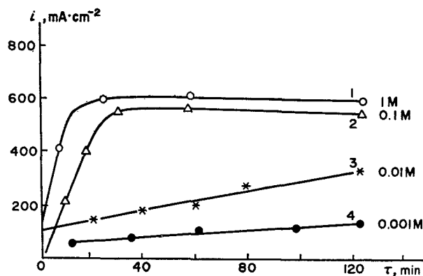
Fig. 2. Dependence of the rate of the cathode evolution of hydrogen under \varphi_r = -0.15 V and 25^\circ\text{C} on the time of treatment of electrode in solution \text{Cd}(\text{NO}_3)_2 .
