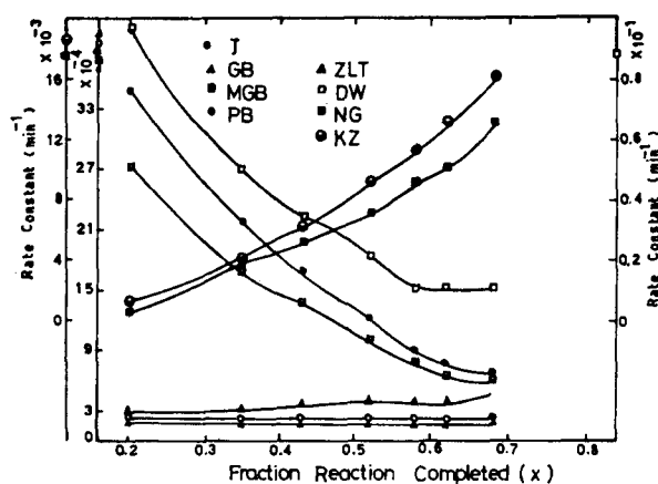
Fig. 2. Analysis of rate constants for 900°C isothermal reaction of ZnO with chromia calculated from: Jander (○), Ginstling-Brounshtein (▲), modified Ginstling-Brounshtein (■), Phase Boundary controlled (●), Zhuravlev-Lesokhin-Tempel (△), Dünwald-Wagner (□), Kröger-Ziegler (⊙) or Nuclei growth controlled (⊠) kinetic equation.
