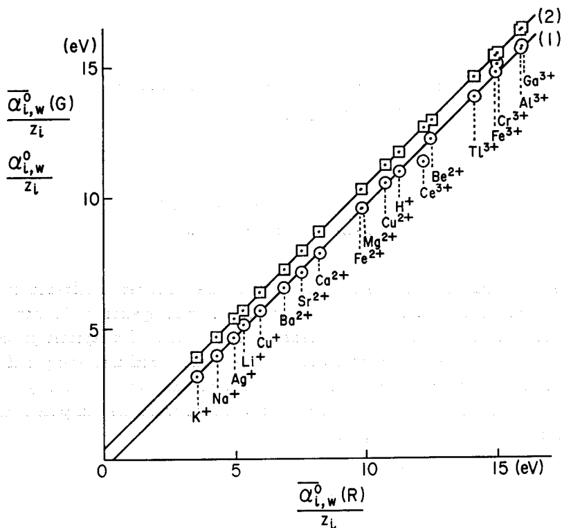
The comparison of the two series of the real free energies of hydration \bar{\alpha}_{i,w}^0(G)/z_i and \bar{\alpha}_{i,w}^0(R)/z_i —the straight line (1), and the relation between the chemical and real free energies of hydration \alpha_{i,w}^0/z_i and \bar{\alpha}_{i,w}^0(R)/z_i —the straight line (2), for monoatomic cations at 25°C.
