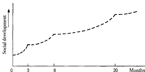
Figure 1 Scallop hypothesis
