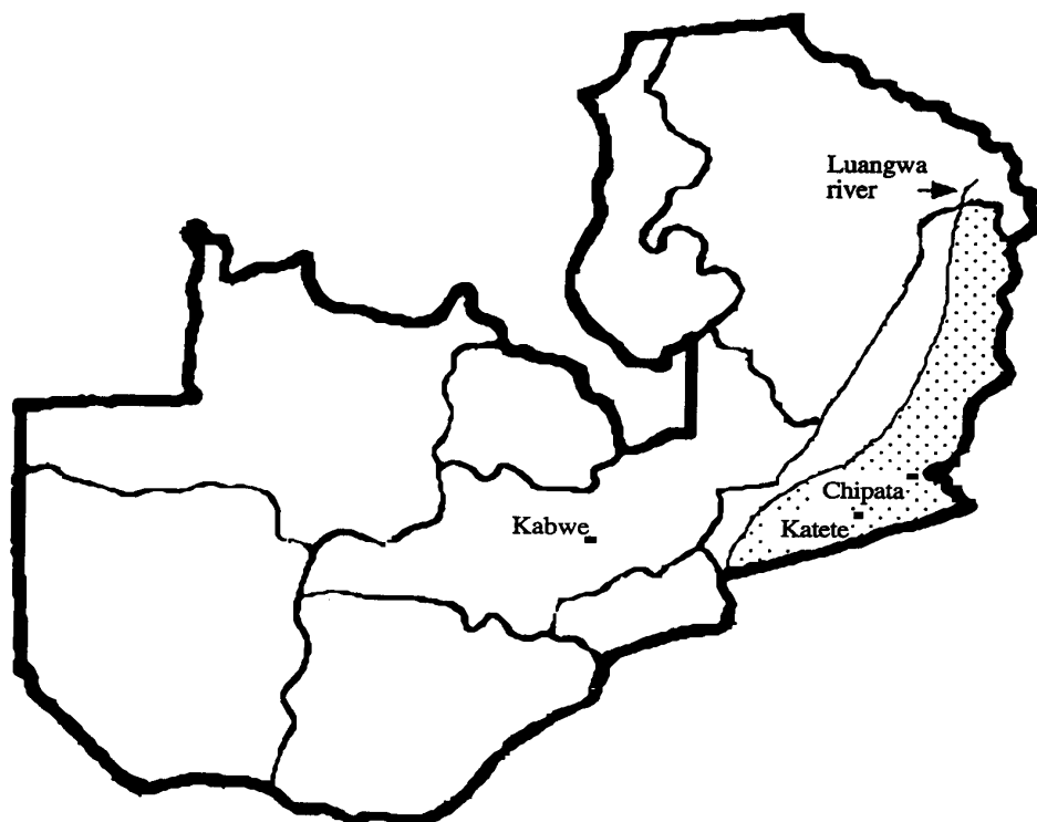
Fig. 1. Map of Zambia showing Kabwe where the ASF outbreak occurred. The shaded area shows part of Eastern province where ASF is endemic.
