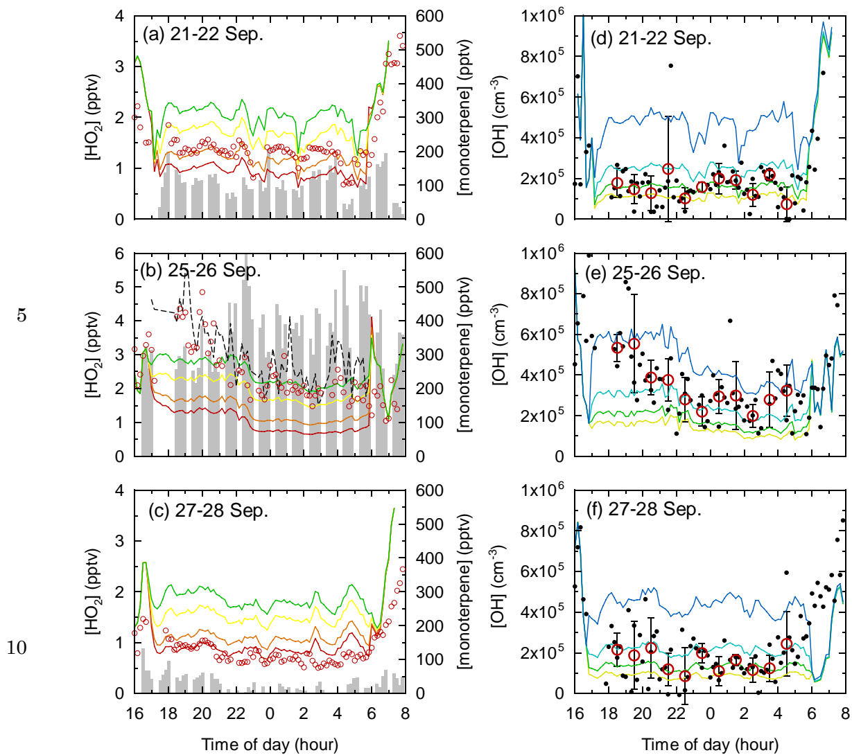
Figure 10. Temporal variations in observed (red circles) and modeled (solid lines) HO 2 and OH concentrations for the three analyzed nights. Red, orange (only in HO 2 plots), yellow, green (in both HO 2 and OH plots), light blue, and blue lines (only in OH plots) correspond to model runs with fixed NO concentrations of 1, 2, 5, 10, 20, and 50 pptv, respectively. The black dashed line for HO 2 on 25–26 September (b) shows the model results where OH concentrations were constrained to the observed 10-min values. The total monoterpene concentrations are shown by shaded bars in the HO 2 plots. The black circles in the OH plots represent 10-min averages. The error bars of the observed hourly OH levels show the 1-σ range for 10-min values included in the hourly data.
