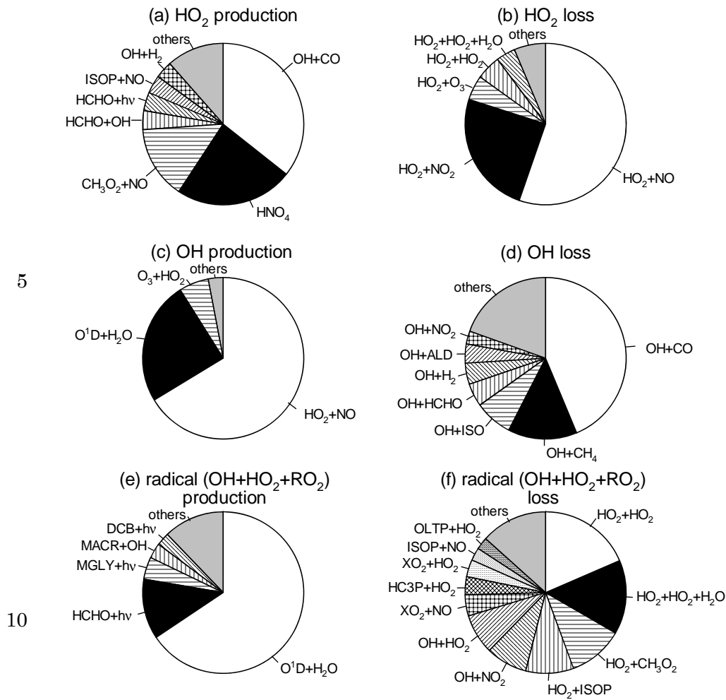
Figure 7. Breakdown of the production and loss processes of HO 2 , OH and the radical group (OH+HO 2 +RO 2 ). Daytime median values (0900–1500 LST) in the base run are used. Species in the model are isoprene (ISO), peroxy radicals formed from ISO and dienes (ISOP), acetaldehyde and higher aldehydes (ALD), methylglyoxal and other \alpha -carbonyl aldehydes (MGLY), methacrolein and other unsaturated monoaldehydes (MACR), unsaturated dicarbonyls (DCB), parametric peroxy radicals that account for additional NO to NO 2 conversions (XO 2 ), peroxy radicals formed from alkanes, alcohols, esters, and alkynes with OH rate constant (298 K, 1 atm) less than 3.4 \times 10^{-12} \text{ cm}^3 \text{ s}^{-1} (HC3P), and peroxy radicals formed from terminal alkenes (OLTP).
