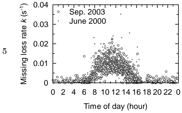
Figure 6. Composite diurnal variations in the missing loss rate of HO 2 ( k ) for September 2003 (open circles) compared to that for June 2000 (gray circles).
