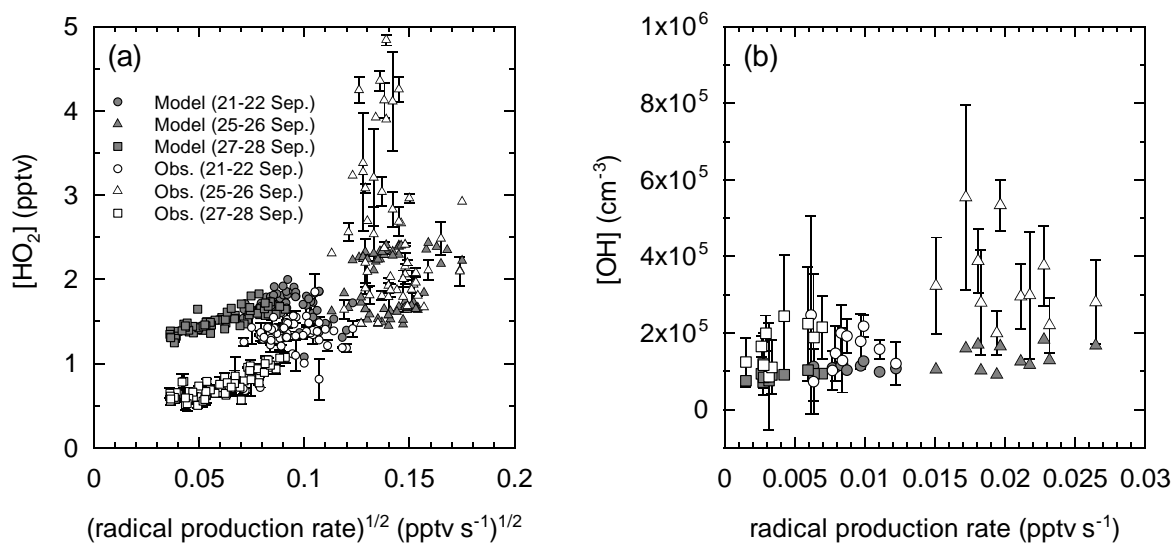
Figure 11. Dependence of observed (open symbols) and modeled (gray symbols) nighttime (a) \text{HO}_2 mixing ratios on square root of radical production rate and (b) OH concentrations on radical production rate. Modeled levels are those for 5 pptv NO. Data for 21–22, 25–26, and 27–28 September are shown by circles, triangles, and squares, respectively. The error bars indicate the 1- \sigma range for 1-min (for \text{HO}_2 ) or 10-min (for OH) values in the 10-min (for \text{HO}_2 ) or hourly (for OH) data.
