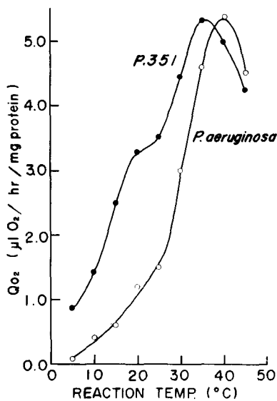
Fig. 2. Effect of temperature on Q_{o_2} values of succinate oxidation by cell-free extracts of P-351 (●) and P. aeruginosa (○). Q_{o_2} was defined as \mu\text{l} of \text{O}_2 uptake per hr per mg of protein.
