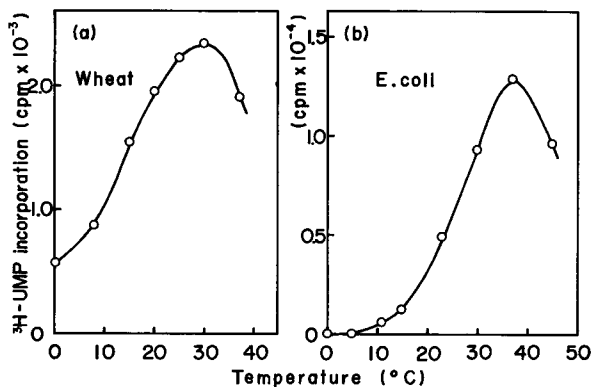
Fig. 4. Optimum temperature for RNA synthesis.
