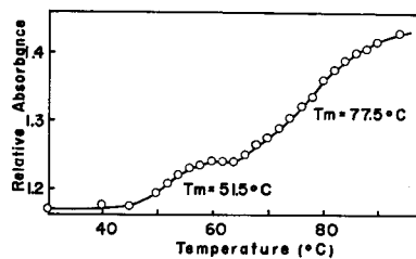
Fig. 2. Melting profile of purified chromatin. Optical density at 260 nm was plotted as a function of the temperature.
