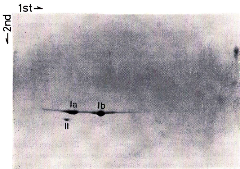
Fig. 2. Two-dimensional electrophoretogram of discoidin subunits. The isoelectric focusing (first dimension) was from the cathode on the left to the anode on the right. The separation by molecular weight (second dimension) was from the cathode at the top to the anode at the bottom. Two discoidin I subunits are indicated as Ia and Ib, and the II indicates the subunit of discoidin II.
