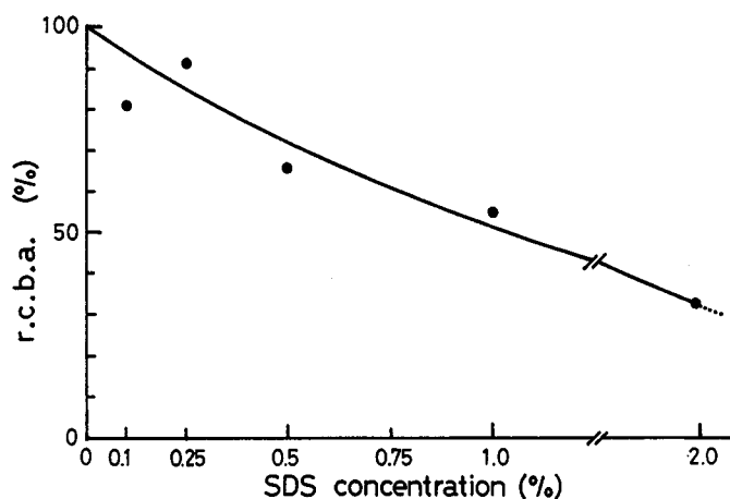
Fig. 3. Effect of SDS on the relative carbohydrate-binding activity of discoidin subunits. The relative carbohydrate-binding activity (r. c. b. a.) was estimated from the protein amount of discoidin subunits specifically bound to Sepharose 4B.
