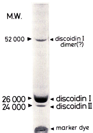
Fig. 1. Electrophoretogram of discoidin subunits in a 10% polyacrylamide gel. Discoidins were isolated and purified by adsorption on a Sepharose 4B column and elution with a buffer containing 0.3 M D-galactose as described in "Materials and Methods". The protein of about 26,000 daltons is the subunit of discoidin I. A minor band of 24,000 daltons is the subunit protein of discoidin II.
