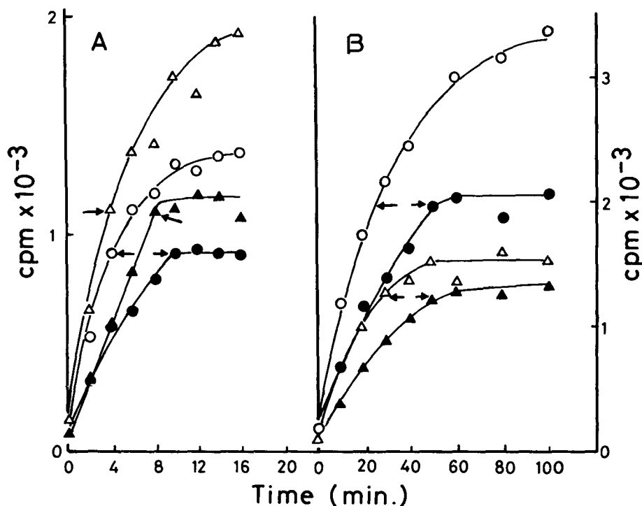
Fig. 2. Purified polysome-directed protein-synthesis. Incorporation of [ 14 C]amino acids was estimated at 25° (A) and 10°C (B) with purified polysome system of P. aeruginosa (△,▲) and V. ABE-1 (○,●) in the absence (△, ○) or presence (▲, ●) of ATA (200 μM for P. aeruginosa and 100 μM for V. ABE-1 ). Supernatant fraction of V. ABE-1 was used in this experiment. Symbol (↔), see the legend to Table 1.
