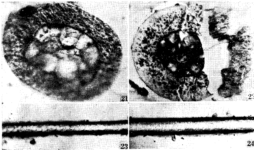
Figs. 1-20. Camera-lucida drawings from cross sections of guard hairs plucked out of various parts of body by way of comparison between two forms of dogs. E; root of the ear. N; neck. Thr; throat. F-b; front-breast. U-b; under-breast. Ab; abdomen. U-Ab; under-abdomen. R; rump. Thi; thigh. Ta; tail.
