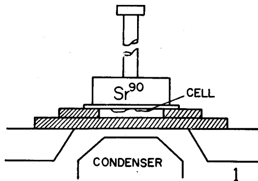
Fig. 1. Schematic diagram illustrating the method of beta-irradiation with a strontium 90 plaque applicator. For details see text.
