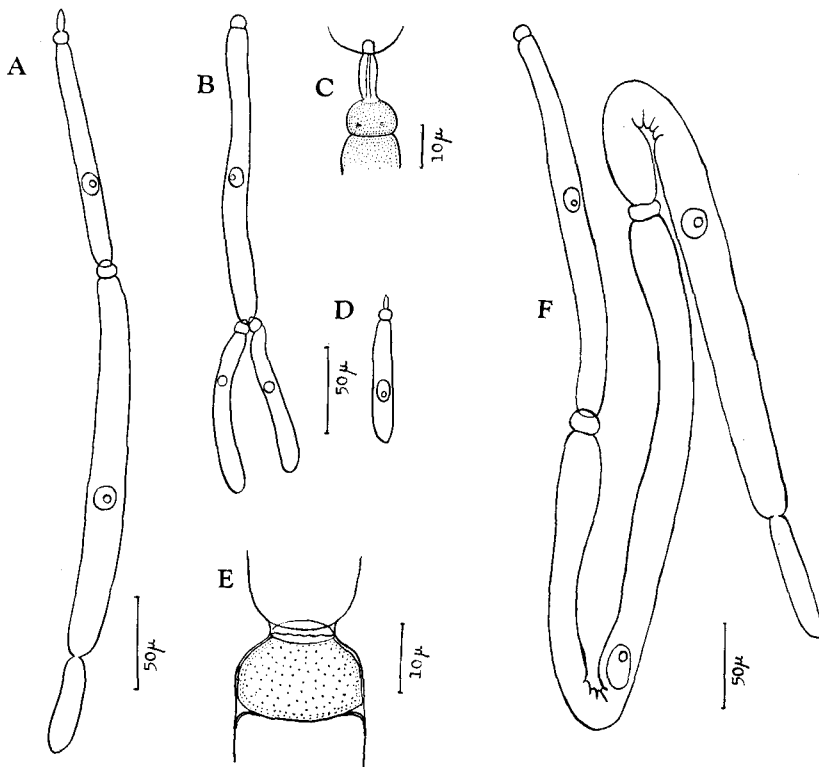
Fig. 2. Uradiophora cuenoti Mercier. A. Associated sporonts. B. Two satellites associated with one primite. C. Epimerite. D. Trophozoite. E. Interlocking region of association. F. Association of three sporonts.
