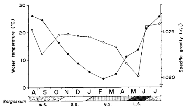
Fig. 2. Seasonal changes of water temperature (solid circles) and specific gravity (open circles) in the Sargassum region.
