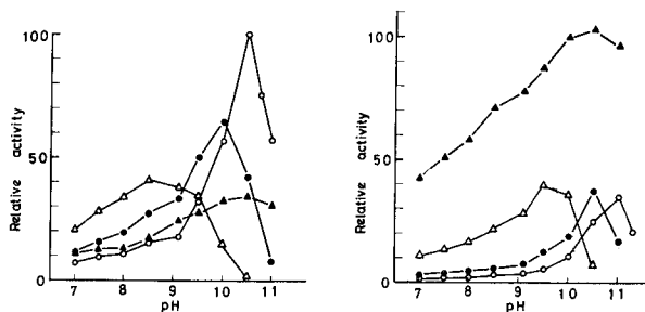
Fig. 8. Effect of pH on crucian carp H6PD. Left, activity with NADP; right, activity with NAD. Substrate and coenzyme concentrations were the same as in Fig. 7. Activity was expressed as percentage of the peak activity with G6P and NADP. ○—○, G6P; ●—●, Gal6P; △—△, dG6P; ▲—▲, glucose.
