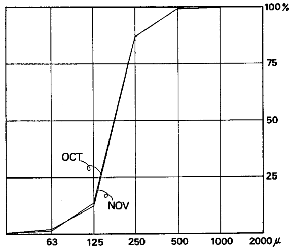
Fig. 2. Cumulative curves of particle size.
