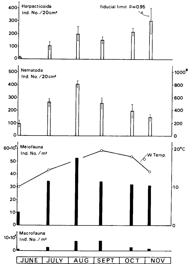
Fig. 3. Temporal fluctuations of individual numbers of Harpacticoida, Nematoda, total meiofauna, and total macrofauna.
