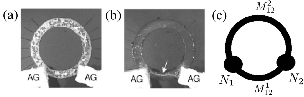
Figure 12: Panels (a) and (b) indicate the initial and final state respectively of the ring-shaped network experiment. The lengths of longer and shorter paths are 42 mm and 13 mm, respectively. The corresponding graph is shown in panel (c), which has two nodes, N_1 and N_2 , and two edges, M_{12}^1 and M_{12}^2 .
