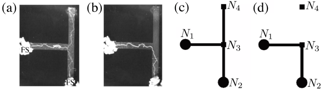
Figure 11: Panels (a) and (b) indicate the initial and final states respectively of the T-shaped graph experiment. Panels (c) and (d) show respectively the initial and the final state of the simulation, which consisted of four nodes and three edges. The width of the black lines reflects the conductivity of each path.
