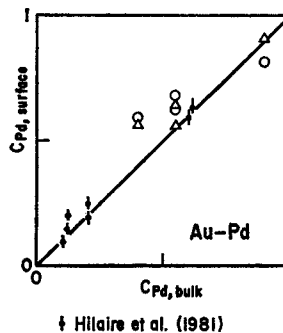
Fig. 2. Surface Pd concentration, as determined from XPS spectra, against bulk (nominal) concentration of various Au-Pd alloys. Data by Hilaire et al. 4) are also shown for comparison.
