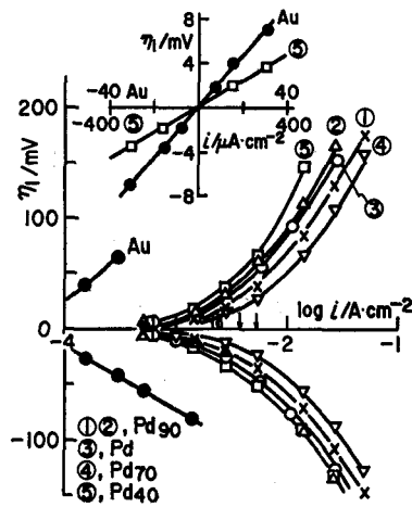
Fig. 4. Plots of \eta_1 against \log i (apparent) on Au-Pd alloy electrodes of various compositions (before the anodic activation) i_{\text{ov}} evaluated from \eta_1 vs. i plots (inset) are indicated by the arrows on the abscissa. Data on the Au electrode are \eta and not \eta_1 .
