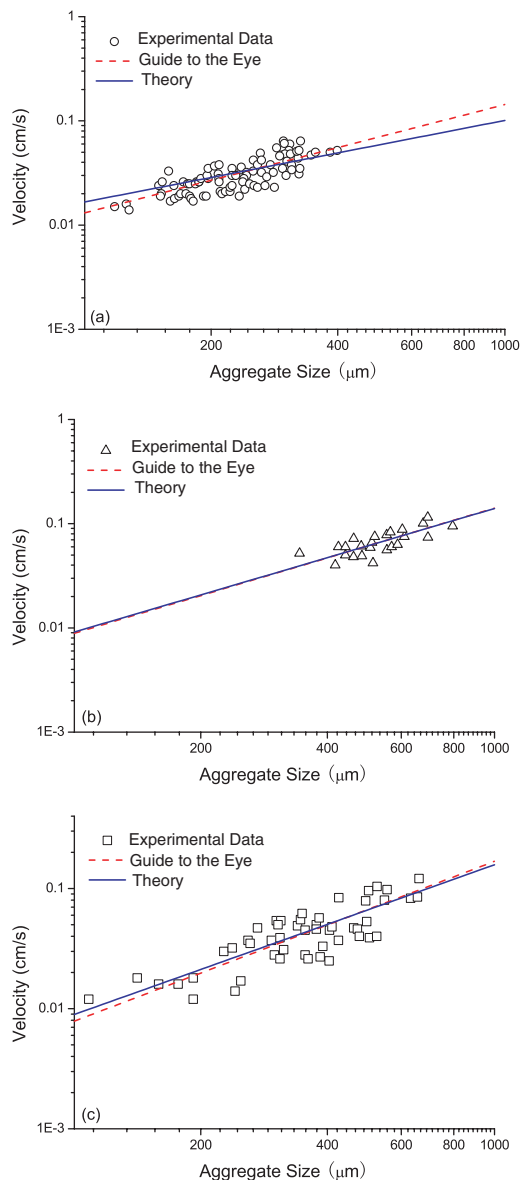
Fig. 1: Settling velocities of aggregates vs. aggregate sizes. The scatters are experimental data taken from ref. [5]. The dashed lines are fitted to experimental data for a guide to the eye. The solid lines are the calculated results according to our theory (eq. (9)) for the cases of (a) D_f = 1.79 , (b) D_f = 2.19 , (c) D_f = 2.25 , respectively. The absolute values of velocities are omitted to give prominence to the power law.
