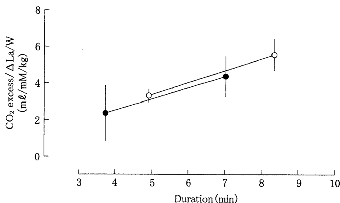
Fig. 2. Relationship between CO_2 \text{ excess}/\Delta La/w and endurance time obtained at each incremental exercise for runners (○) and untrained men (●).
