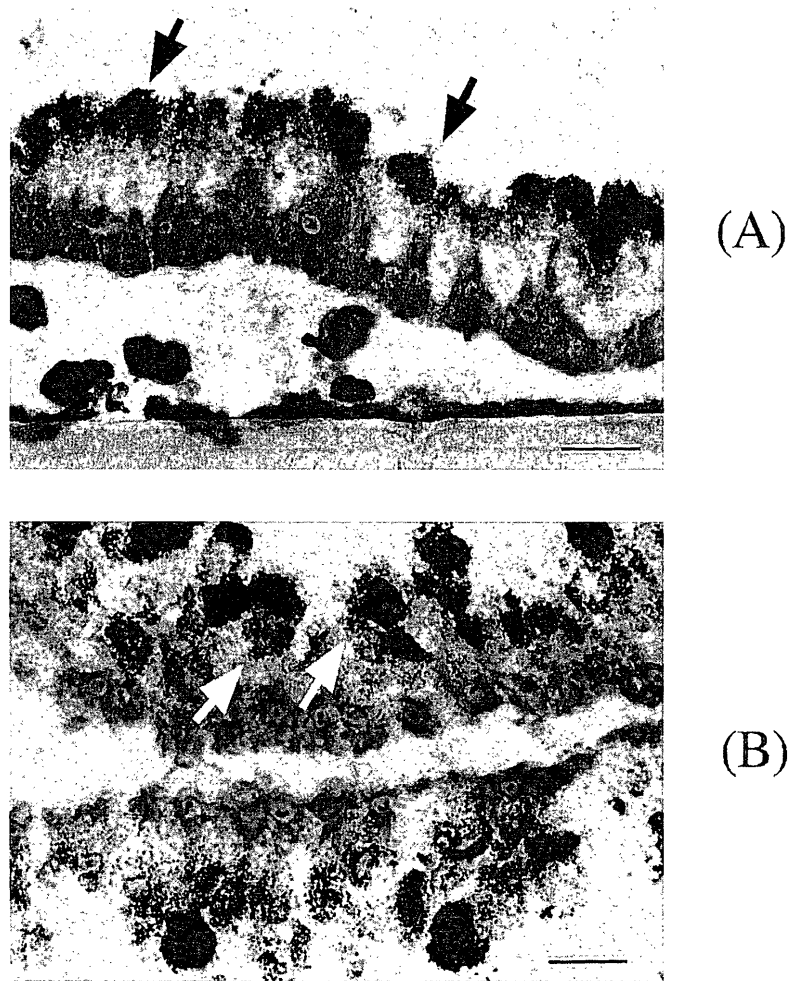
Fig. 3 Toluidine blue-stained sections showing the destruction of midgut cells.
