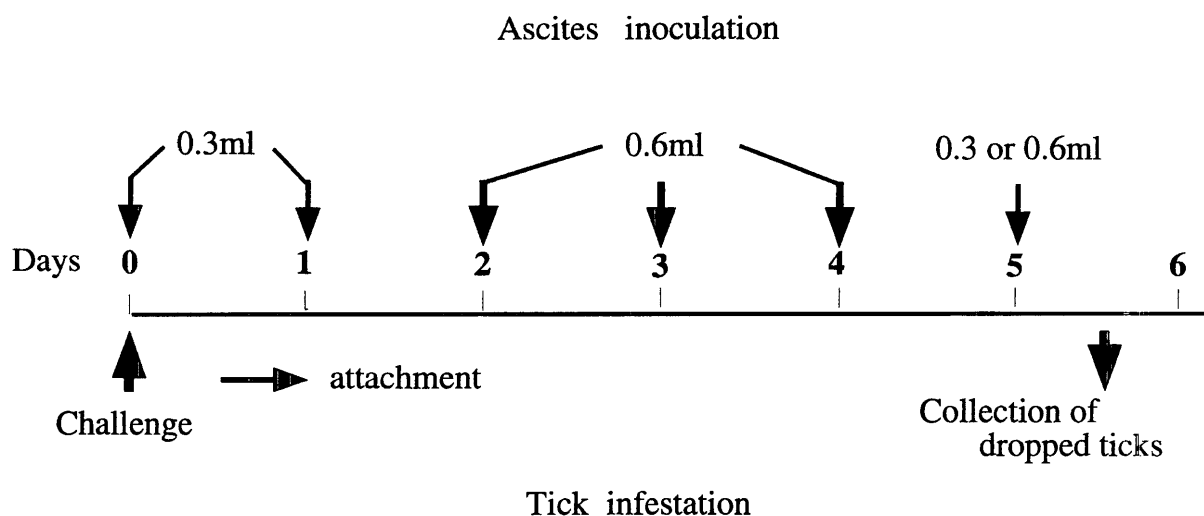
Fig. 1 Schematic representation of passive immunization. Ascites of each isotype mAb was diluted to contain at least 50 \mu\text{g}/0.3 \text{ ml} of IgG, and mice were immunized with 0.3 or 0.6 ml of ascites every day, as a high dose mAbs test (described in Materials and Methods). In a similar way, a low dose test was conducted. Each IgG concentration was adjusted to 20 \mu\text{g}/0.2 \text{ ml} , and mice were immunized with 0.2 or 0.4 ml of ascites every day.
