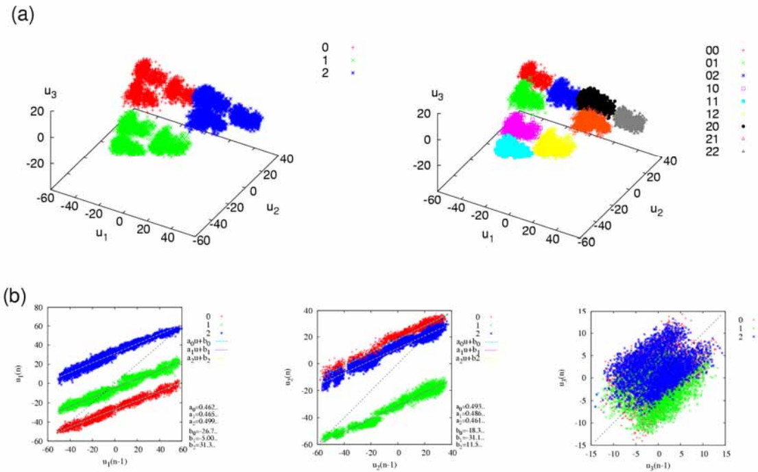
Figure 1 A cantor coding in the phase space constructed by membrane potentials of CA1 model neurons. Three different spatial patterns are repeatedly input from the CA3 to the CA1 neurons in a random order. (a) Self-similar structures are shown in the phase space. Each color indicates the input sequence of length one (left), and of length two (right). Principal Component Analysis is applied to the state vectors, and the principal components up to the third are shown. The states of the CA1 are hierarchically clustered in a self-similar manner according to the input sequences. (b) Return maps of each principal component. In each figure, return maps corresponding to different inputs are represented by different colors. In the first and second components, the maps are well described by contractive affine transformations, which indicates an appearance of the IFS-like dynamics producing fractal structure of the membrane potentials.
