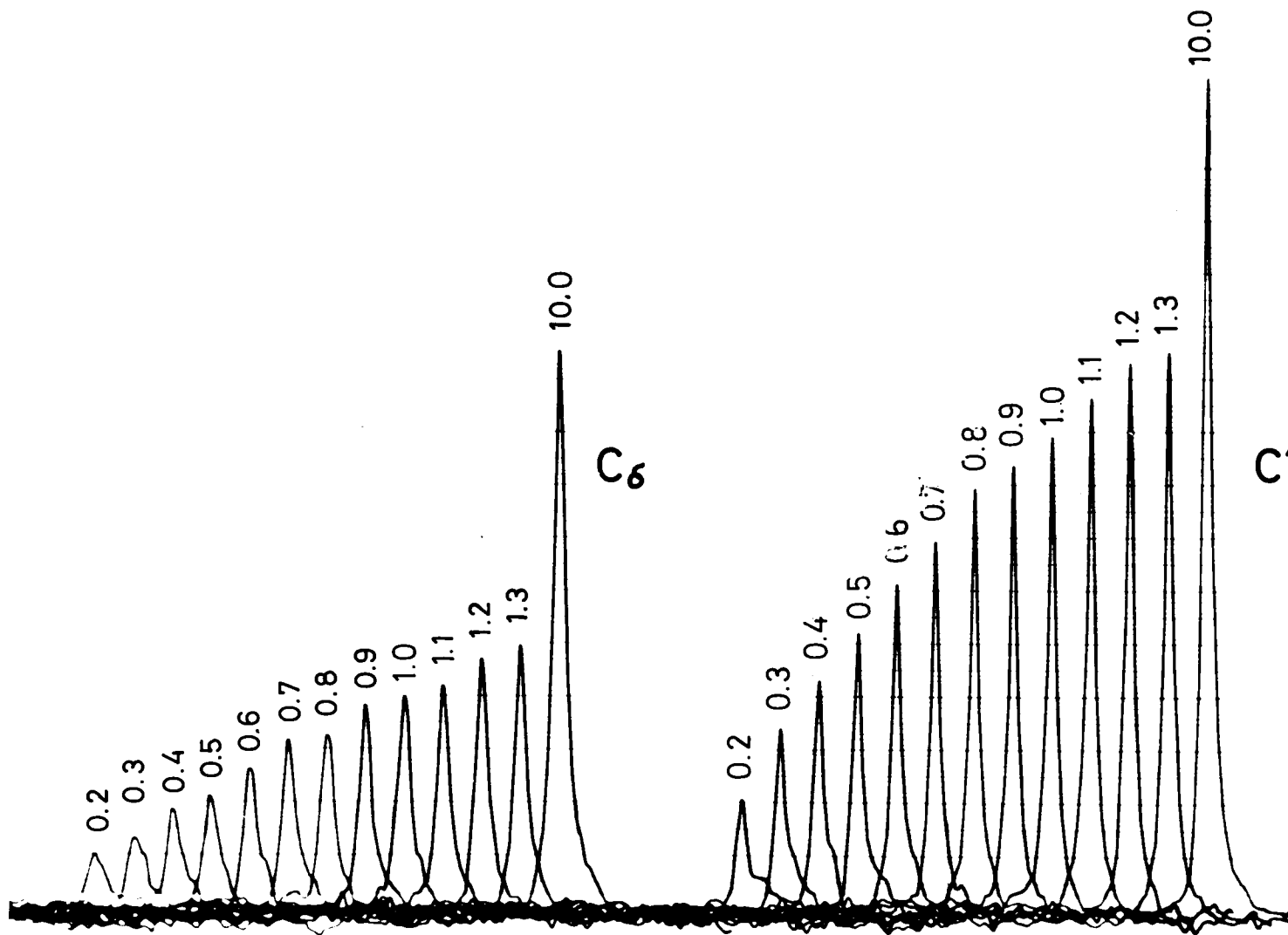
Figure III-4. ^{13}\text{C} saturation recovery Fourier transform NMR spectra of \text{C}_6 and \text{C}' carbons at pH 5.3. Each spectrum is the result of 2048 scans with a waiting time of 1.86 sec. The delay time is shown at the top of each spectrum in seconds.
