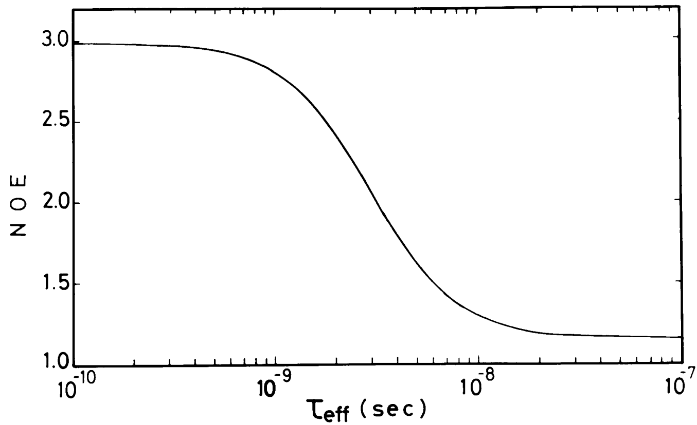
Figure III-9. Semilog plot of NOE vs. \tau_{eff} . See caption of Figure III-8 for other details.
