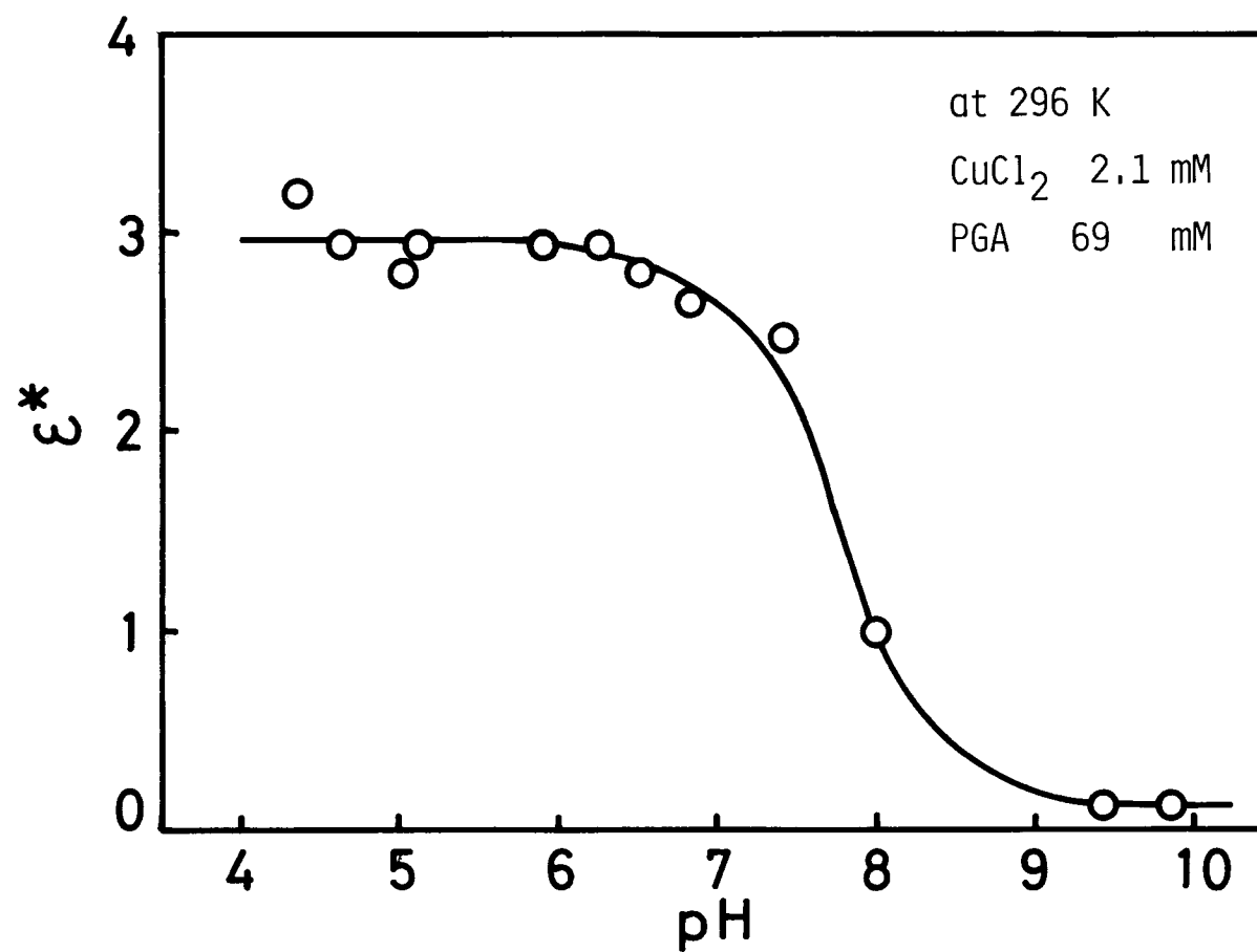
Figure IV-6. pH dependence of water-proton relaxation enhancement factor \epsilon^* at 296 K: [\text{Cu(II)}]=2.1 mM, [\text{PGA}]=69 mM. All samples were prepared with 0.2 M NaCl solution.
