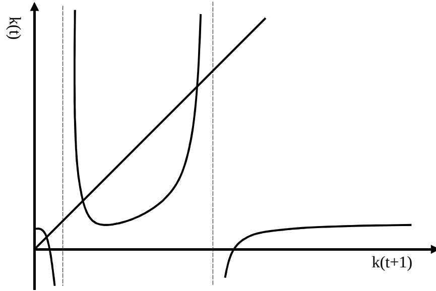
Figure 4-3a. Function W : Case with (1 - \phi\theta) \beta_H - \beta_L > 0
