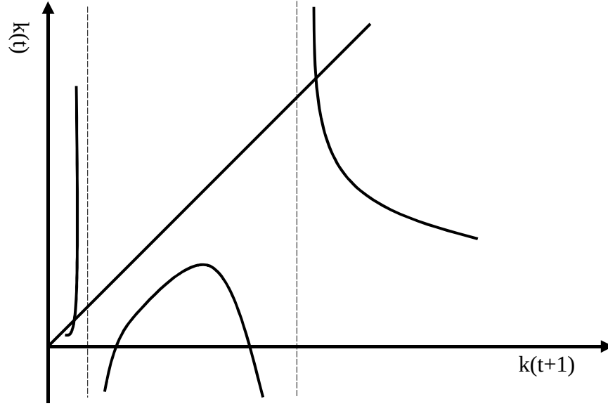
Figure 4-3b. Function W : Case 2
