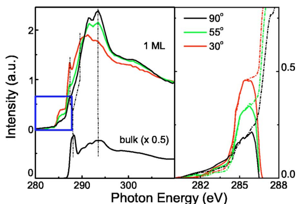
FIG. 1. (Color online) Experimental result for the C K -edge NEXAFS spectra in 1 ML C_{44}H_{90} (TTC) films grown on Cu(001) for the x-ray incidence angle \theta varied over 30^\circ , 55^\circ , 90^\circ . We also display for comparison the result for a multilayer TTC (bulk) on Cu(001) in black (which is almost \theta independent, here for \theta=90^\circ ). All the spectra are normalized by their edge jump. Right-hand panel is a blowup of the prepeaks, obtained by subtracting the bulk (multilayer) spectrum which has no structures at the edge onset.
