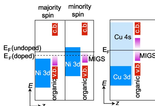
FIG. 5. (Color online) A schematic energy diagram for MIGS in organic/Ni and in organic/Cu.
