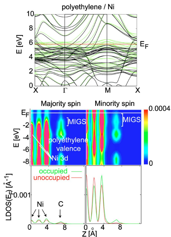
FIG. 3. (Color online) A plot similar to Fig. 2 for 1 ML polyethylene/Ni(001), where the spin density functional theory is adopted. Green (black) lines in the band structure represent the majority (minority) spin.
