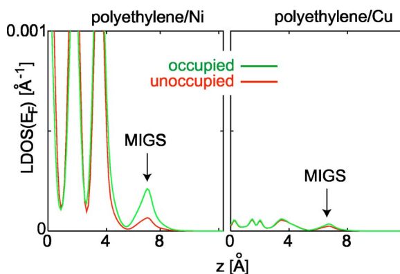
FIG. 4. (Color online) Theoretical results for the local density of occupied and unoccupied states at E_F are compared for polyethylene/Ni and polyethylene/Cu.
