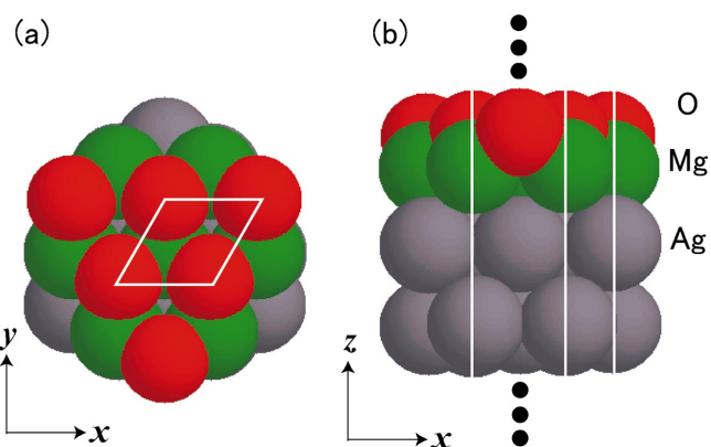
FIG. 2. (Color) Top (a) and side (b) views of the atomic configuration considered in the present study. The unit cell is indicated in white.
