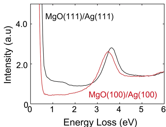
FIG. 1. (Color) EELS result, with the primary-electron energy of 60 eV, for the one MgO(111) layer on Ag(111) as compared with that for MgO(100) on Ag(100).
