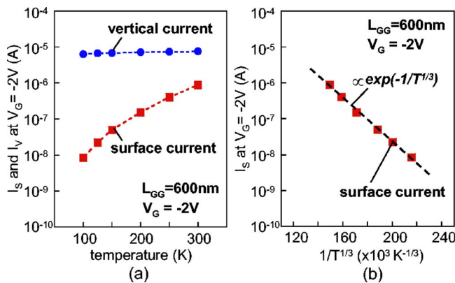
FIG. 3. (Color online) (a) Temperature dependences of I_s and I_v at V_G = -2 V and (b) I_s at V_G = -2 V as a function of 1/T^{1/3} showing a straight line, consistent with 2D-VRH conduction.
