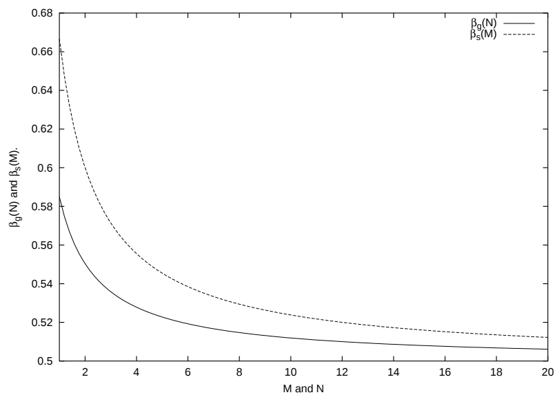
Figure 5: Critical values of \beta ; \beta_g and \beta_s .
