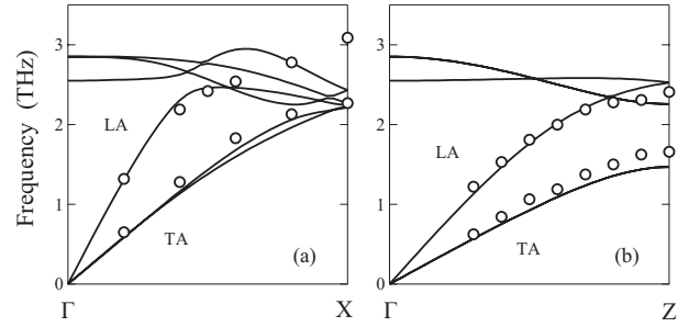
FIG. 2: Phonon dispersion relations (below about 3 THz) in \text{CaWO}_4 , (a) in the \Gamma -X direction and (b) in the \Gamma -Z direction. The experimental (circles) [12] and calculated (solid lines) frequencies for the transverse acoustic (TA) and longitudinal acoustic (LA) branches are compared.
