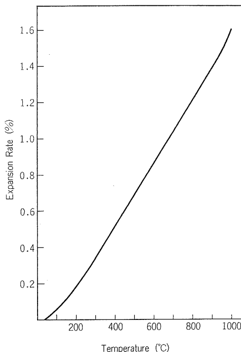
Fig. 13 Expansion curve of Ni-30 wt% Ta.
