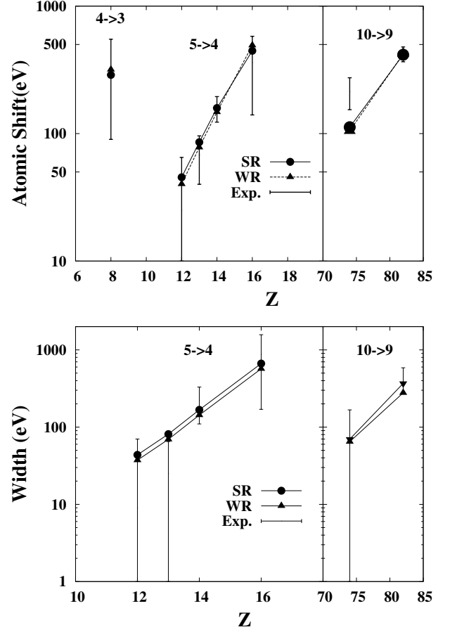
Fig. 3. Atomic shift and conversion width of \Sigma^- .
