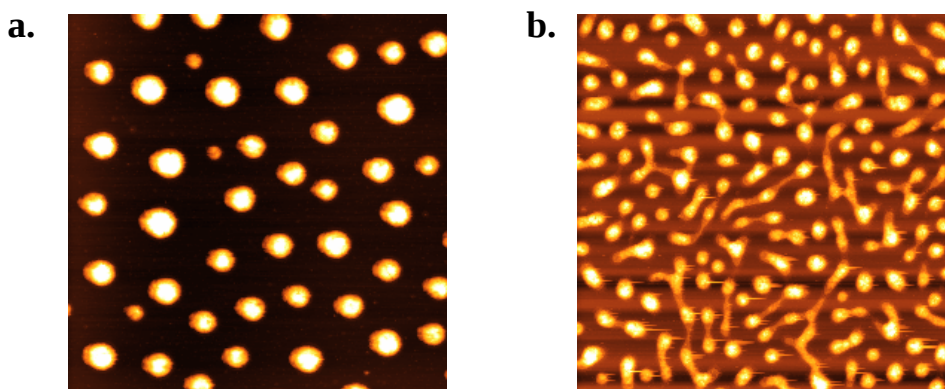
Figure 1. Nanodot structures of cast-films of 1 - (I_2)_2 . Surface morphology of nanodots on a) bottom and b) top area of mica. The size of images are 10 x 10 \mu\text{m} .
