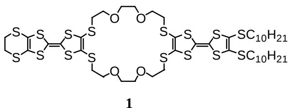
Scheme 1. Molecular structure of ethylenedithio-substituted bis-TTF annulated macrocycle 1 .
