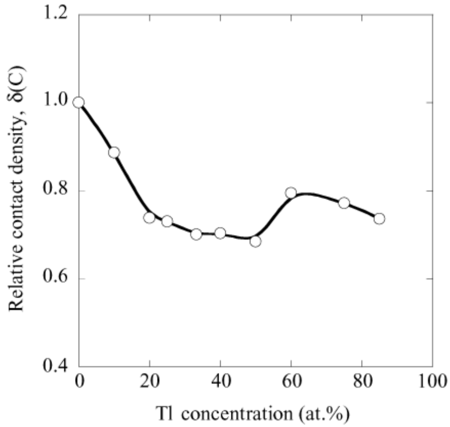
Fig. 4 The concentration dependence of the relative contact density at {}^7\text{Li} nucleus, \delta(C) , for liquid Li-Tl alloys at the temperature 10K higher than the liquidus temperature. The line is the fitted curve. The error is discussed in the text. The error is within the size of data points.
