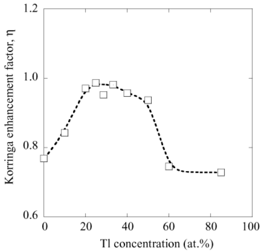
Fig. 5 The concentration dependence of the Korringa enhancement factor for liquid Li-Tl alloys at 793K. The line is the aide for the eye. The error is within the size of data points.
