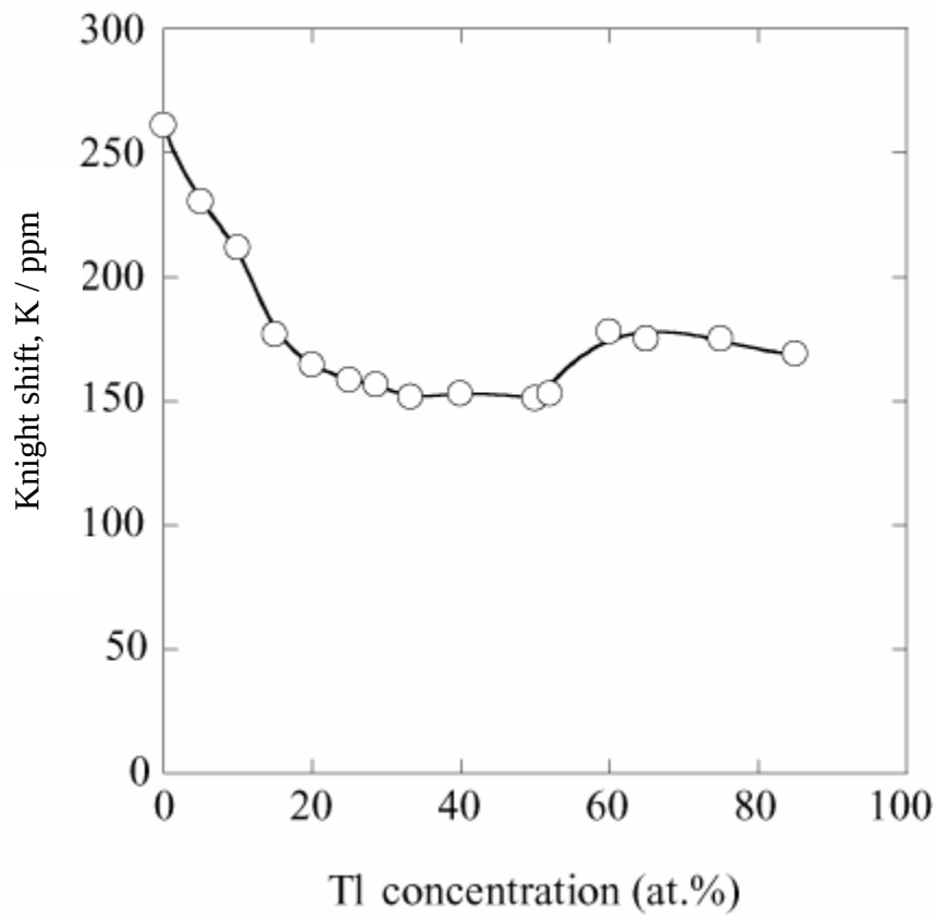
Fig. 1 The concentration dependence of the ^7\text{Li} Knight shift, K , for liquid Li-Tl alloys at the temperature 10K higher than the liquidus temperature. The line is the fitted curve. The error is within the size of data points.
