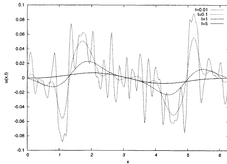
(a) Plot of the solution \omega(x, t) up to t = 5
