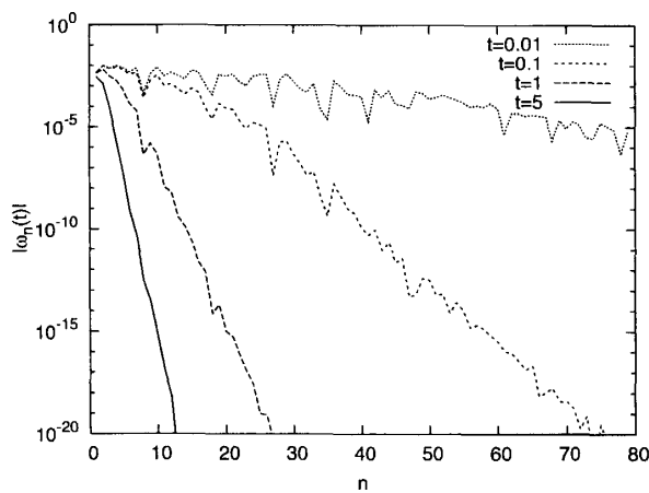
(b) Log plot of the Fourier coefficients |\omega_n(t)|
