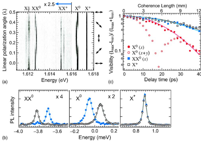
FIG. 1. (Color online) (a) PL intensity contour plot as a function of the linear polarization angle. The data were collected by the depolarized excitation at the WL excitation (5 K, 0 T). The PL polarization is depicted to the right of the figure. (b) PL spectra of the three main peaks XX^0 , X^0 , and X^+ at a linear polarization angle of 0 and \lambda/4 , which are x (open circles)- and y (solid circles)-polarized PL components, respectively. Note that the energy axis is replotted from the midpoint of the two peaks of X^0 . Clear fine structures are observed in the X^0 and XX^0 spectra, and no fine structure is observed for X^+ . The linewidths (full width at half maximum) are 40, 75, and 40 \mu\text{eV} for XX^0 , X^0 , and X^+ , respectively. (c) Typical visibility plot of the PLs of X^0 , XX^0 , and X^+ at WL excitation. x or y in the parentheses indicates the polarization of the PL component. The solid lines are the fitting curves.
