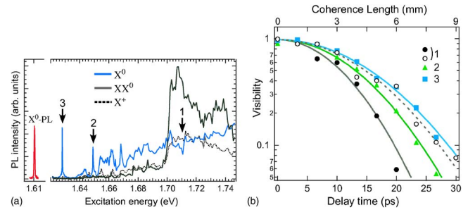
FIG. 2. (Color online) (a) PL excitation spectra at the detection energy of X^0 . (b) Visibility plots of the PLs of the neutral exciton X^0 at different excitation energies: WL (solid circles) and 1 LO-resonant (triangles and squares) excitations. The respective excitation energies correspond to 1, 2, and 3 in (a). Only the x -polarized component was detected. The solid lines are the fitting curves.
