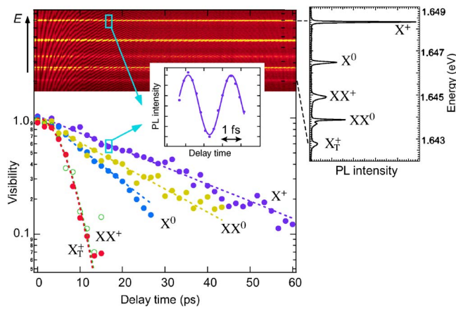
FIG. 3. (Color online) Visibility plot of the PLs of exciton and exciton complexes from the same single QD at WL excitation (5 K). The dashed lines are the fitting curves. The raw interferogram (upper panel) and the time-integrated spectra (right panel) are also shown.
