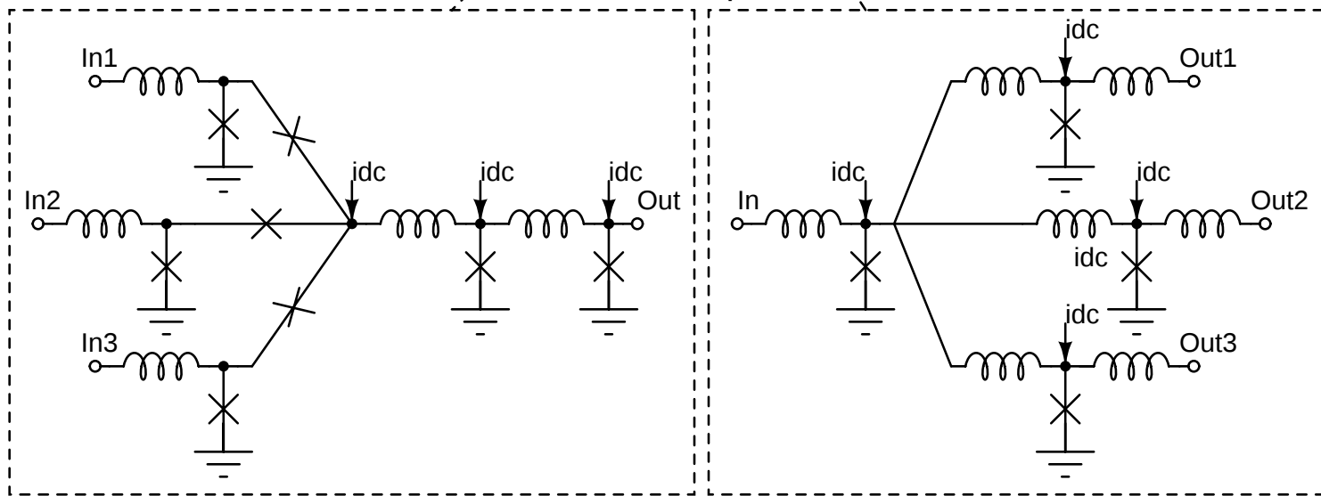
Splitter
