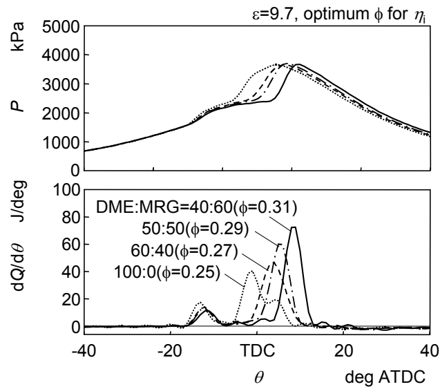
Fig.4 Indicator diagrams of HCCI combustion of DME and MRG.
