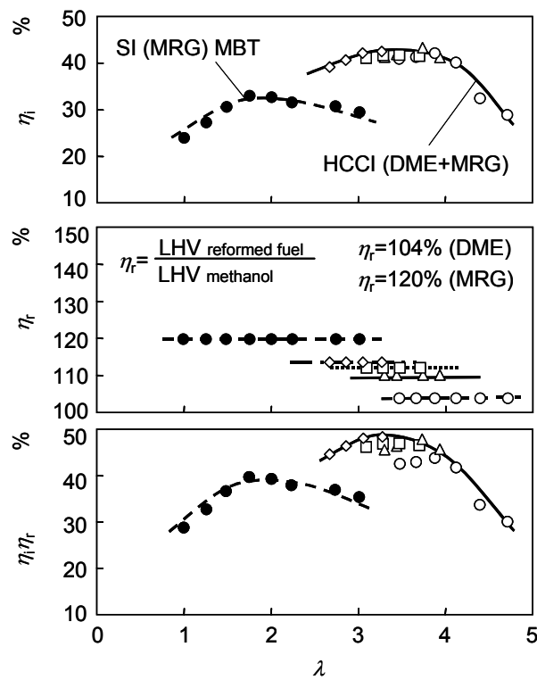
Fig.10 Overall thermal efficiency of HCCI combustion and SI combustion based on methanol.
