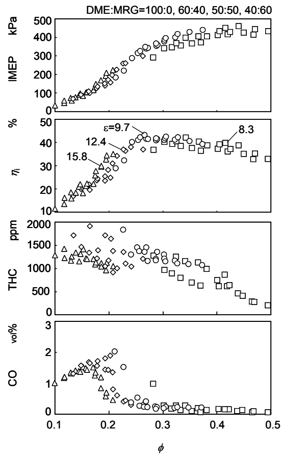
Fig.5 HCCI combustion of DME and MRG for different compression ratios (DME:MRG=100:0,60:40,50:50,40:60).
