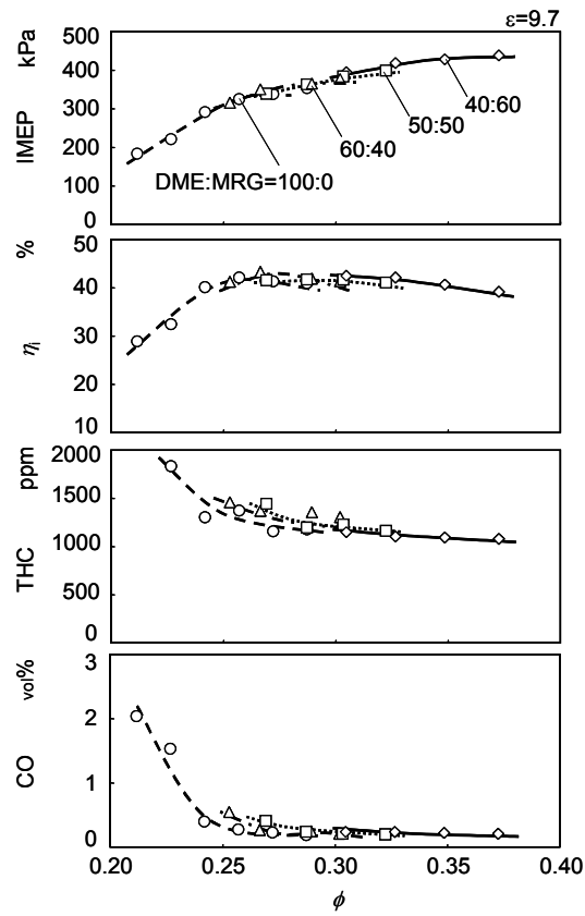
Fig.3 Indicated mean effective pressure, indicated thermal efficiency and exhaust emissions in HCCI combustion of DME and MRG.
