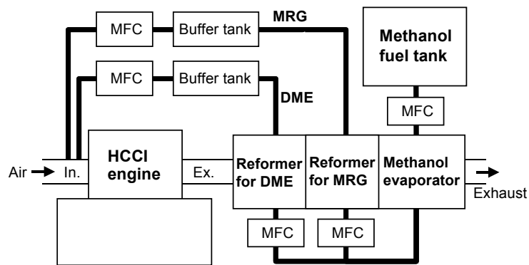
Fig.1 Proposed system of HCCI combustion engine fuelled with DME and MRG onboard-reformed from methanol.
