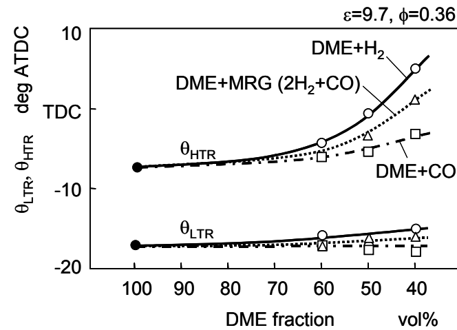
Fig.12 Crank angles at the beginnings of first and second stage heat releases.
