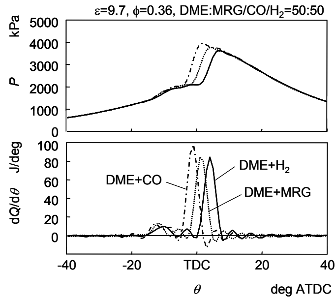
Fig.11 Influences of hydrogen, carbon monoxide and MRG on HCCI combustion of DME.
