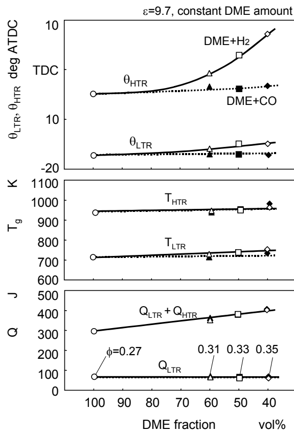
Fig.15 Comparison of effects by hydrogen and carbon monoxide at a constant DME amount.
