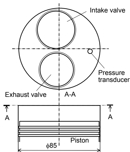
Fig.2 Combustion chamber of tested engine.
