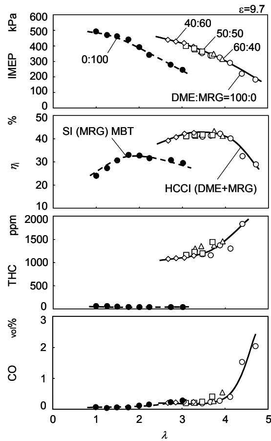
Fig.8 Comparison of SI combustion and HCCI combustion.
