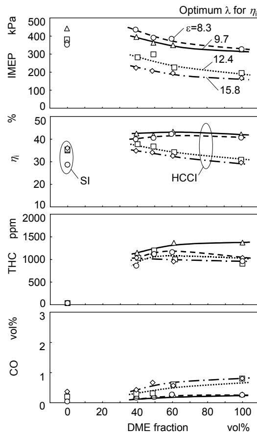
Fig.9 Comparison of SI combustion and HCCI combustion for different compression ratios.
