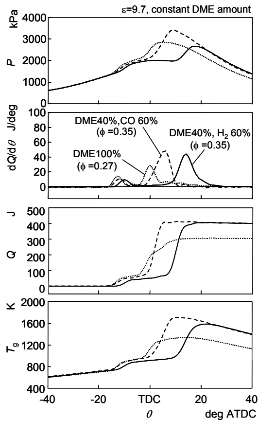
Fig.14 Comparison of effects by hydrogen and carbon monoxide at a constant DME amount.
