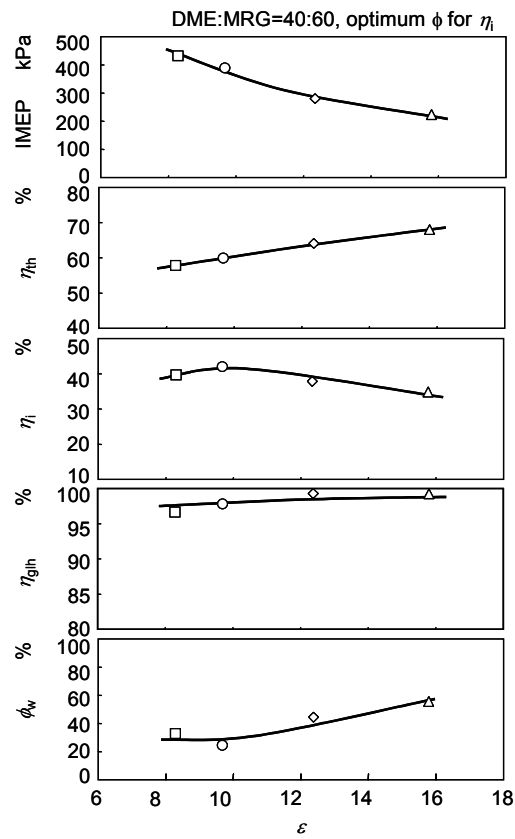
Fig.7 Influence of compression ratio on thermal efficiency factors.
