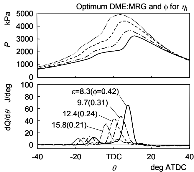
Fig.6 Indicator diagram of HCCI combustion for different compression ratios.
