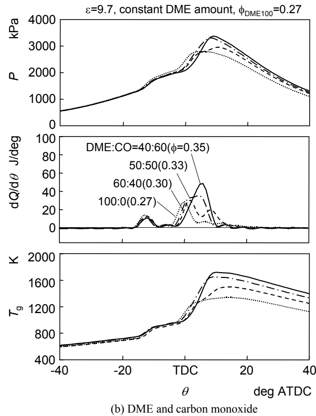
Fig.13 Influences of hydrogen and carbon monoxide on HCCI combustion of DME at a constant DME amount.
