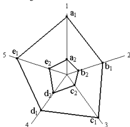
Fig. 1. Graphical representation of the form, components and size of the environmental resource utilization coefficient (ERUC) using a petal-diagram.
