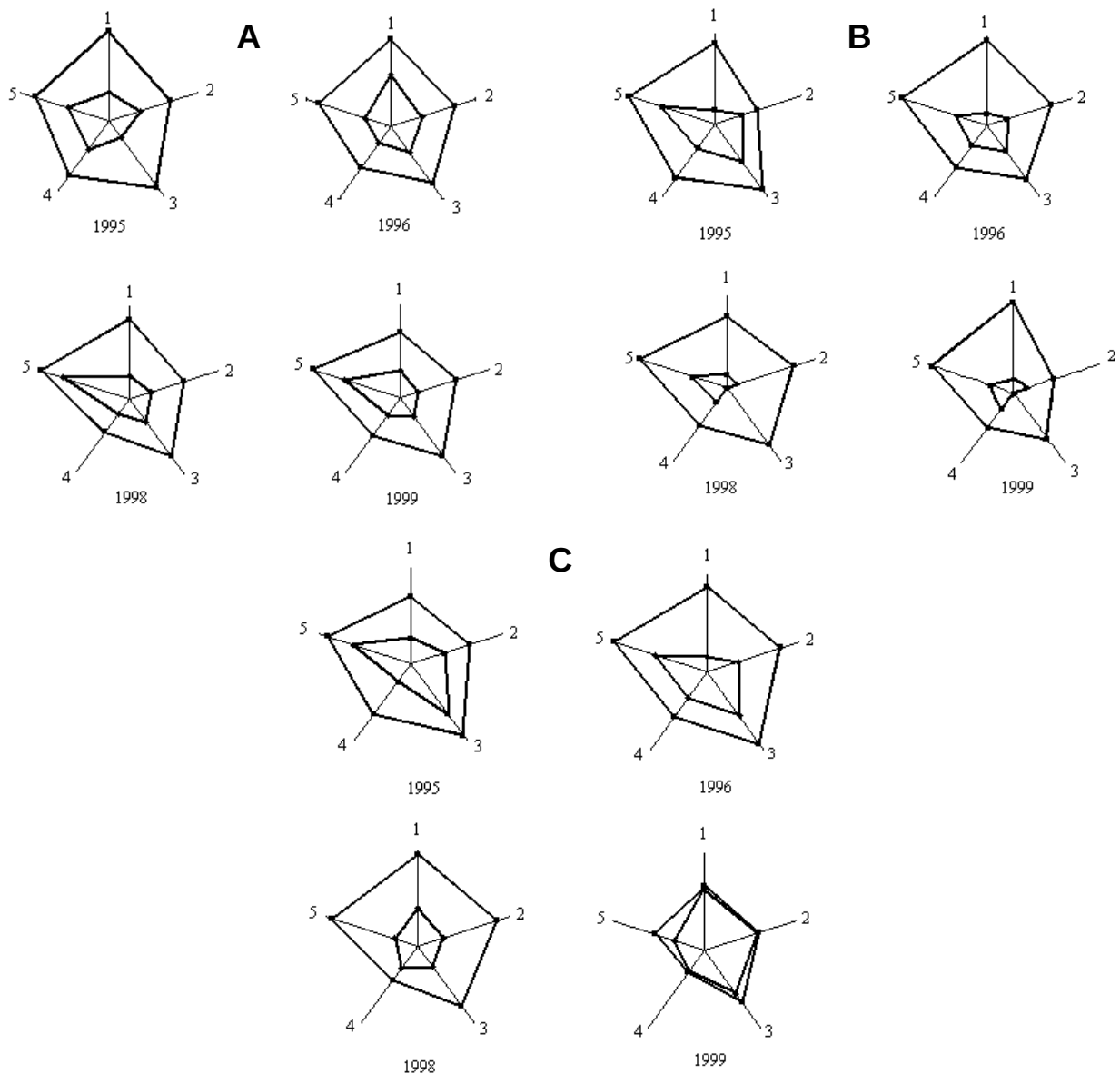
Fig. 2. A – ERUC for common pine, B – for Siberian spruce, C – for Siberian larch.
