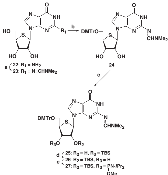
Scheme 2. (a) N,N -dimethylformamide dimethyl acetal, DMF; (b) DMTrCl, pyridine; (c) TBSCl, imidazole, pyridine; (d) Et 3 N, MeOH; (e) N,N -diisopropylmethylphosphonamidic chloride, i Pr 2 NEt, DMAP, CH 2 Cl 2 .
