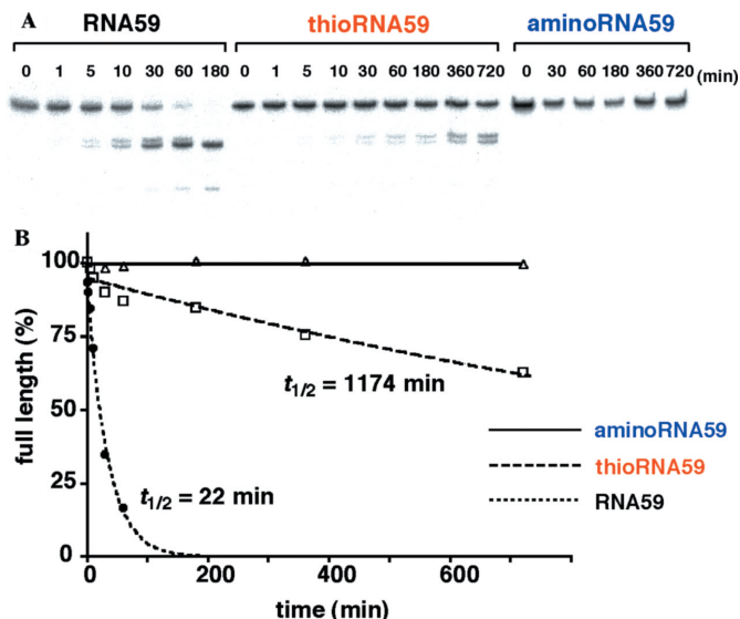
Figure 6. Stabilities of RNA59 , thioRNA59 and aminoRNA59 toward RNase A. (A) PAGE analysis of labeled RNAs incubated at 37°C in the presence of RNase A. (B) Time course of degradation of RNAs by RNase A.
