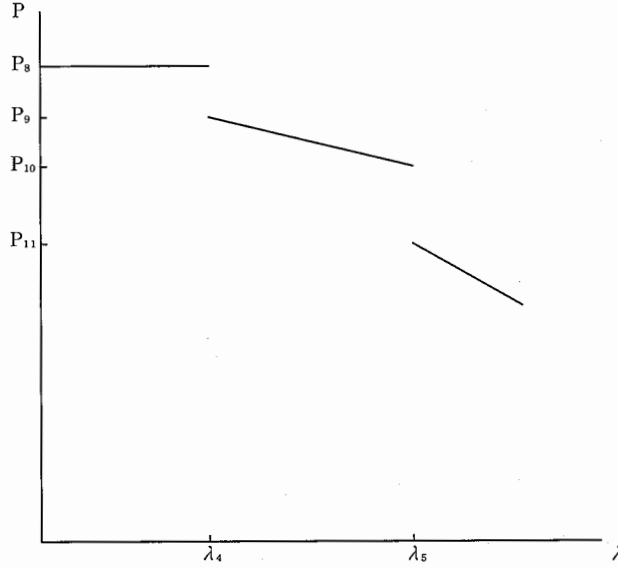
Figure 4. ( S > 9/4 )
