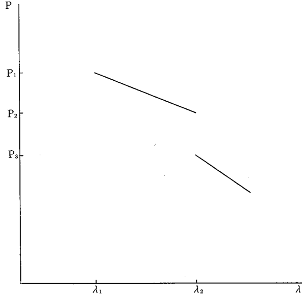
Figure 2. ( 0 < S < 1 )
