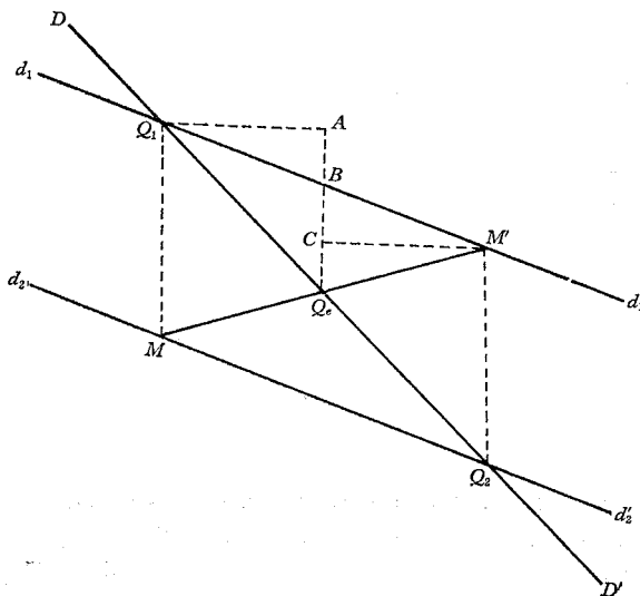
Figure 7. A Critical Position of the Objective Demand Curve in the Case of Optimistic Expectation
