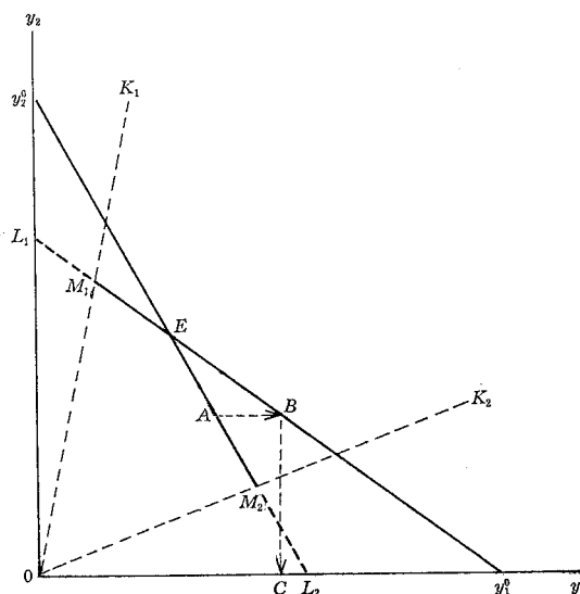
Figure 12. Unstable Duopolistic Equilibrium of Two Optimistic Entrants
