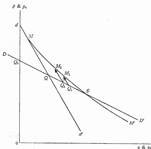
Figure 10. Unstable Equilibrium on the U-Shaped Maximal Curve
